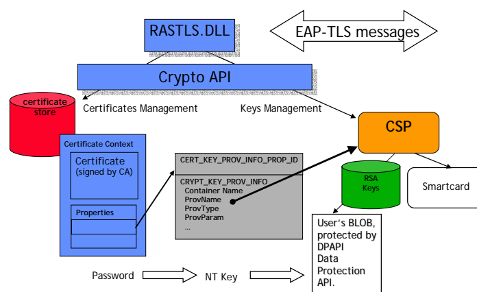
Figure 2 : Architecture EAP-TLS sous Windows.
