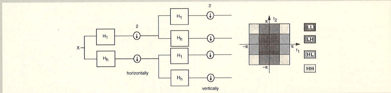
Fig. 17. Separable two-dimensional filter bank corresponding to a separable wavelet basis with resolution change by 4 (2 in each dimension). The partition of the frequency plane is indicated on the right. H_l and H_h stand for low-pass and high-pass filter, respectively.
