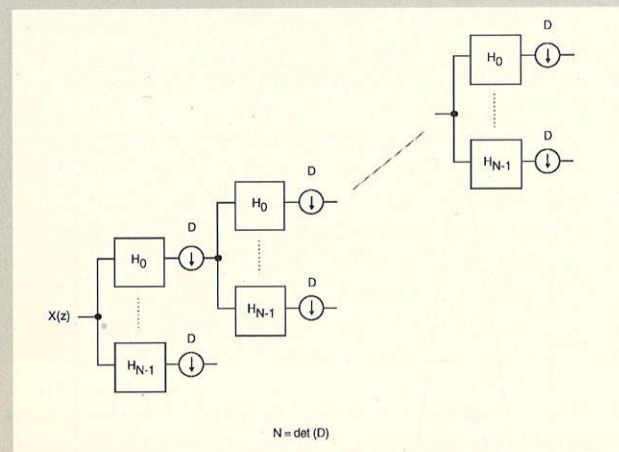
Fig. 18. Iteration of a non-separable filter bank based on non-separable subsampling. This construction leads to non-separable wavelets.
