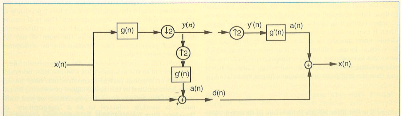
Fig. 10. Pyramid scheme. Derivation of a lowpass, subsampled approximation y(n) , from which an approximation a(n) to x(n) is derived by upsampling and interpolation. Then, the difference between the approximation a(n) and the original x(n) is computed as d(n) . Perfect reconstruction is simply obtained by adding a(n) back.
