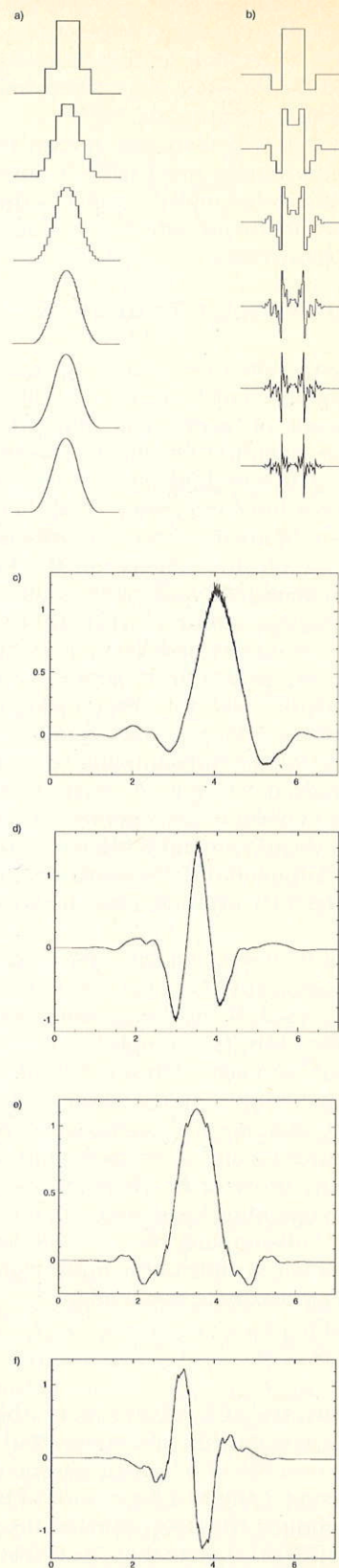
Fig. 12. (a) Iterated low-pass filter g_j(n) with g(n) = (1,3,3,1) , converges to a regular, smooth function. (b) Iterated low-pass filter with g(n) = (-1,3,3,-1) converges to a fractal function (see text). (c) Smith and Barnwell 8-tap lowpass filter [SMI86], iterated 8 times. Divergence occurs, due to rapid oscillations in the temporal waveform. (d) Corresponding continuous-time wavelet (after [RIO90b]). (e) Johnston 8-tap lowpass filter [JOH80], iterated 8 times. The limit function is not differentiable. (f) Corresponding continuous-time wavelet.
