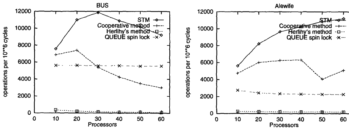
Figure 7: Resource Allocation Benchmark
