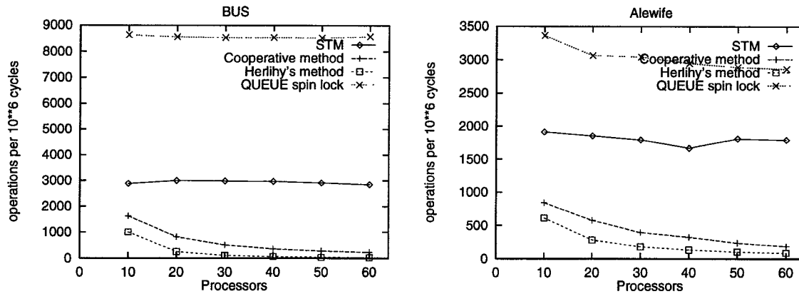
Figure 9: Doubly Linked Queue Benchmark
