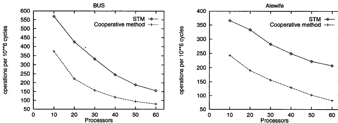
Figure 10: Non-blocking implementations of Israeli & Rappoport's Priority Queue
