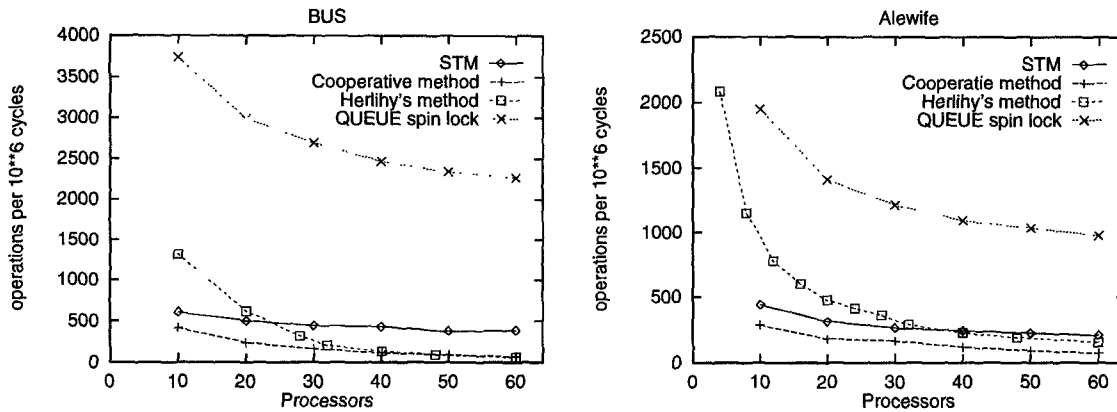
Figure 8: Priority Queue Benchmark
