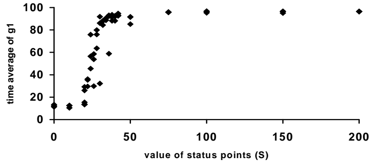
Figure 6: Influence of the status-to-vitality conversion coefficient S . Analysis performed through 64 runs of 3000 generations each. For each run, the time average of g_1 is computed and its value is plotted. Experiments have been concentrated around the cut-off value.
