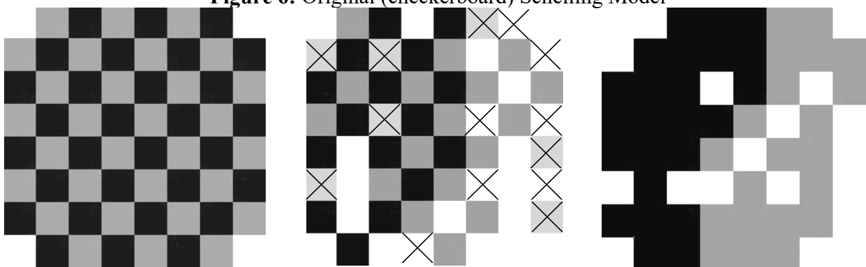
Figure 6: Original (checkerboard) Schelling Model
