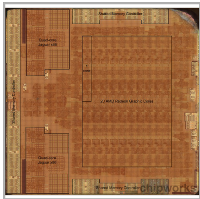
APU PS4 (18 × 19 mm 2 ) TSMC 28 nm, http://www.chipworks.com
