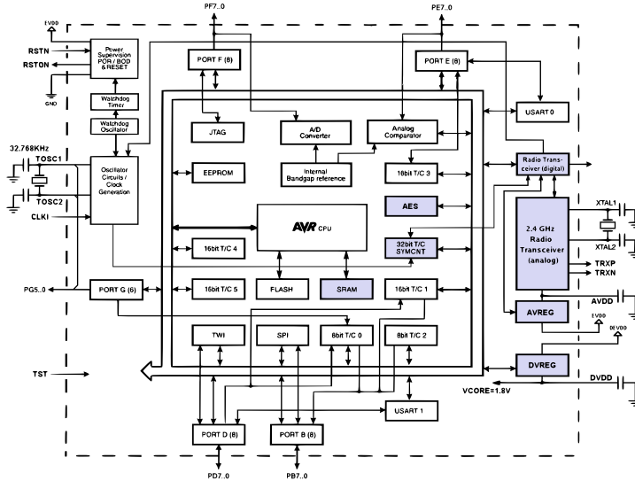
ATmega 128RFA1
