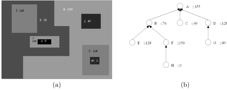
FIGURE 2.1. Example of FLST : (a) Synthetic image ; (b) Inclusion tree obtained with FLST.
