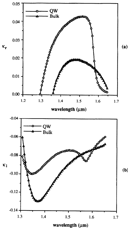
Fig. 1. The real (a) and imaginary (b) parts of \kappa at a carrier density of 3 \times 10^{18} \text{ cm}^{-3} as a function of wavelength for an \text{In}_{0.53}\text{Ga}_{0.47}\text{As}/\text{InP} bulk laser and an \text{In}_{0.53}\text{Ga}_{0.47}\text{As}/\text{In}_{0.72}\text{Ga}_{0.28}\text{As}_{0.6}\text{P}_{0.4}/\text{InP} quantum well (QW) laser with well thickness equal to 10 nm. Other parameters are given in Table 1.
