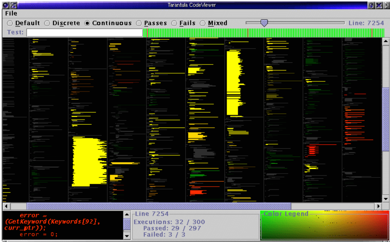
Figure 1. A screen snapshot of the TARANTULA system in Continuous mode.
