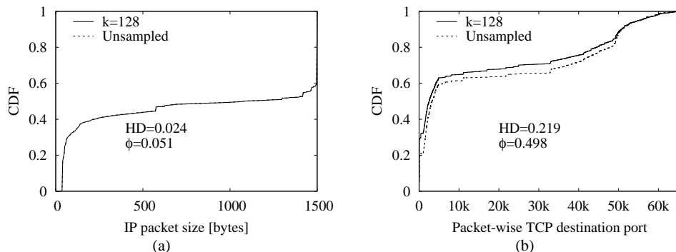
Figure 2. Example of distortion of aggregate features (Campus dataset): CDF of IP packet size (a) and number of packets per destination TCP port (b). Plots report the CDF gathered from the unsampled vs sampled traffic aggregate (systematic sampling, k = 128 ), along with the statistical indexes of distortion.
