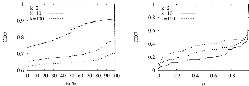
Figure 8. CDF of (left) Err% and (right) \rho for UniBS trace and different sampling step.
