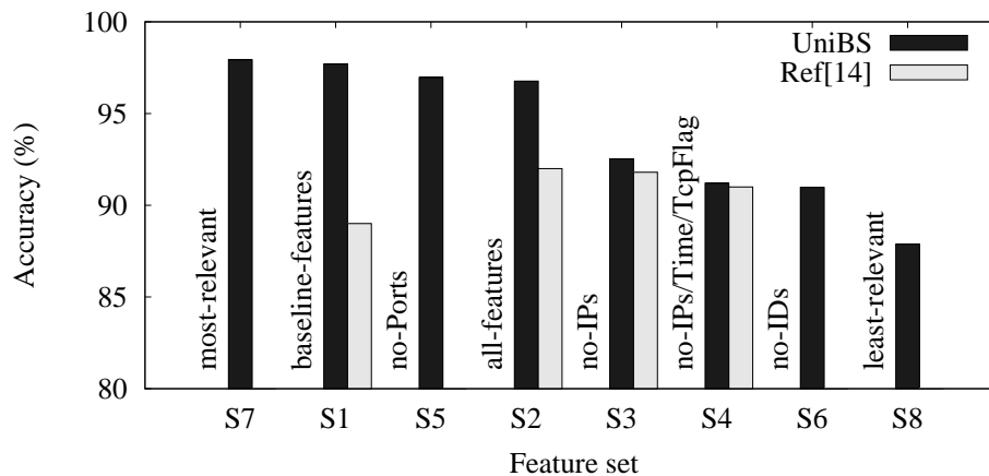
Figure 11. Classification accuracy achieved by different features sets with unsampled traffic for UniBS trace.
