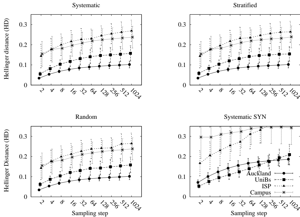
Figure 7. Mean and variance of the HD distortion score for the robust group of features as a function of the sampling step for different sampling policies.
