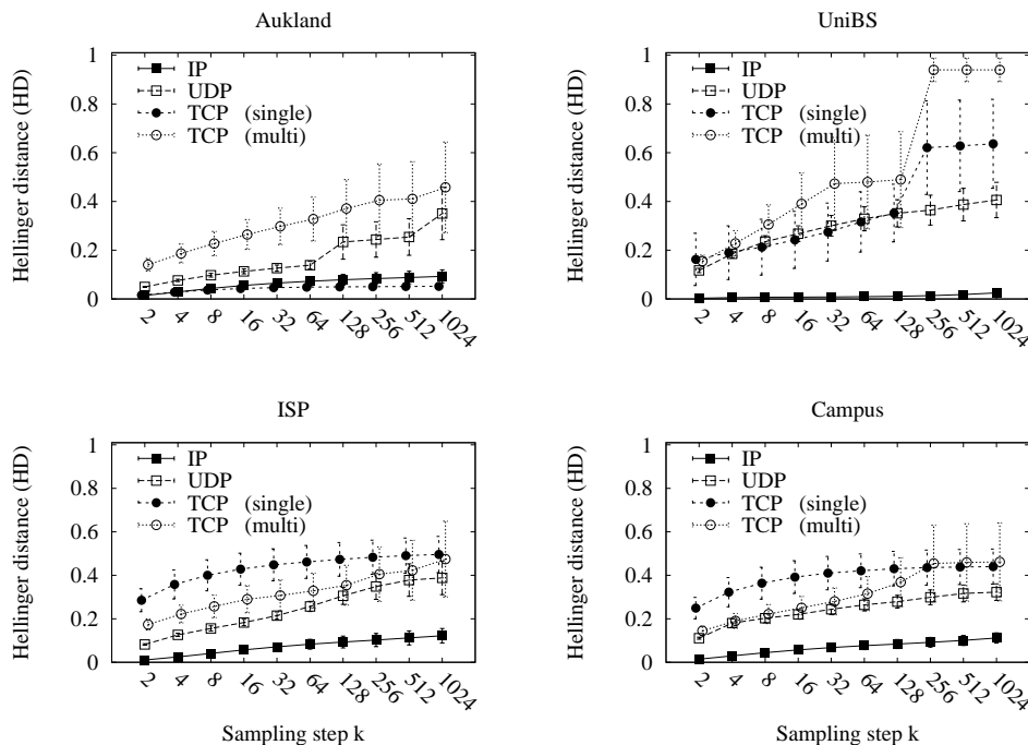
Figure 6. Mean and variance of the HD distortion score, for features grouped by protocol layer, as a function of the sampling step under uniform sampling policy. The extremely low distortion of “TCP single” features in the Auckland trace is an artifact due to the lack of packet payload, in particular of TCP options.
