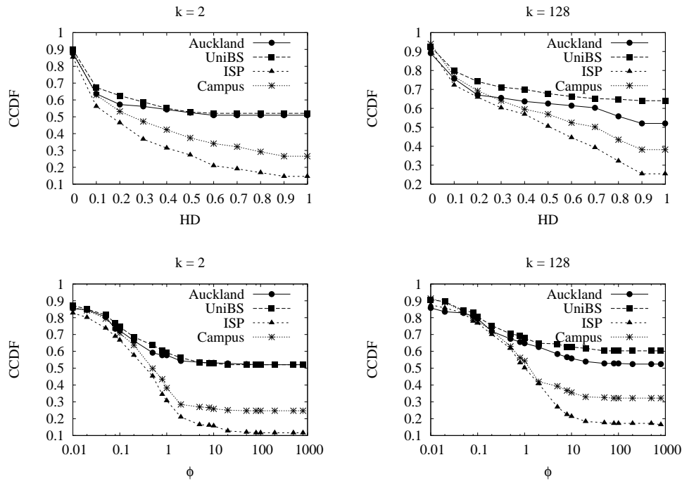
Figure 4. Distribution of the Hellinger distance and \phi coefficient over the whole features set for systematic sampling and k \in \{2, 128\} .
