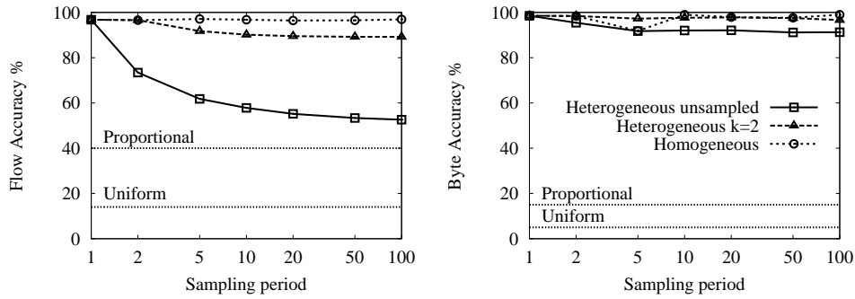
Figure 12. Impact of Homogeneous vs Heterogeneous training set policies at varying sampling rates in terms of flow and byte accuracy.
