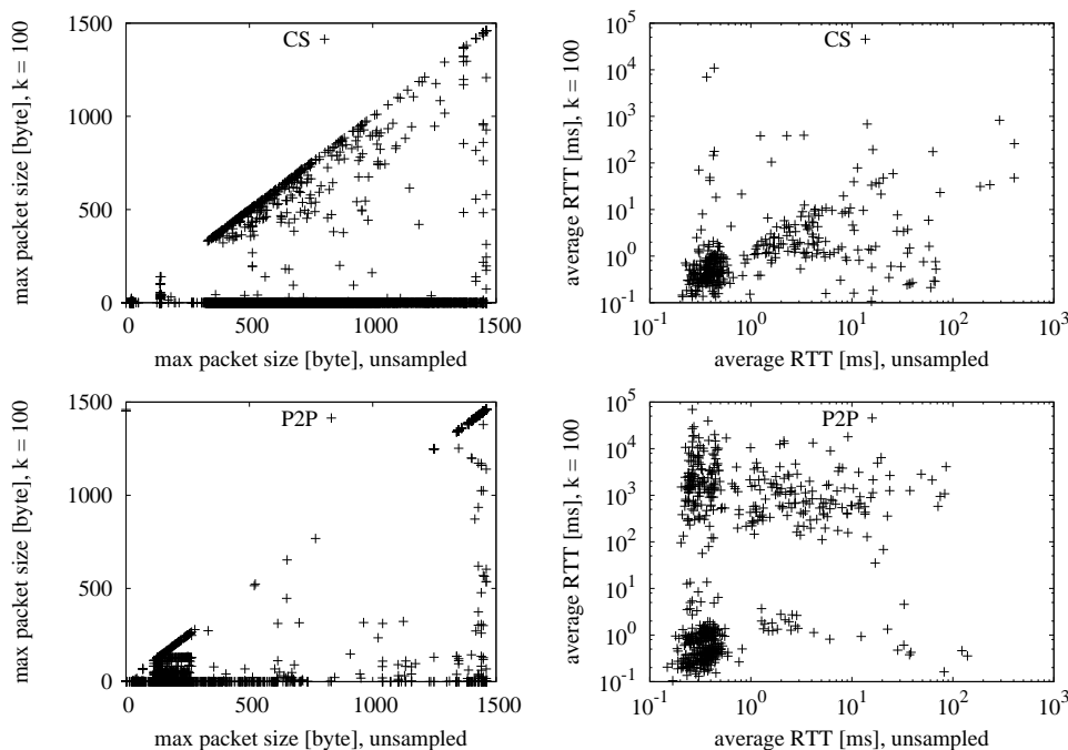
Figure 9. Scatter plot of features values for unsampled and SYN Sampling k = 100 for UniBS trace, contrasting peer-to-peer (P2P) and traditional client-server (CS) applications.
