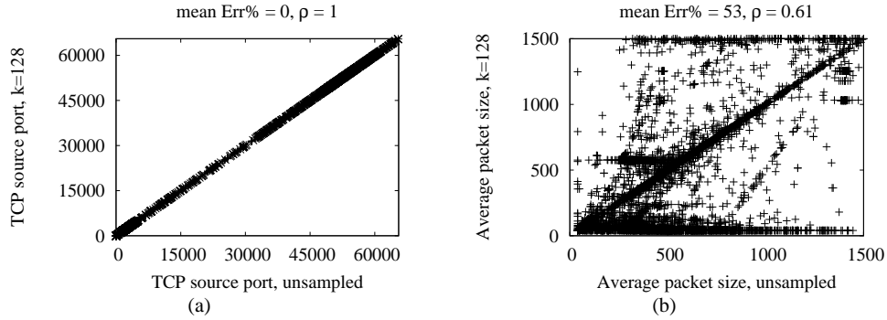
Figure 3. Example of distortion of per-flow features (Campus dataset): scatter plot of TCP source port (a) and average packet size (b) for unsampled vs sampled traffic, along with statistical indexes of correlation.
