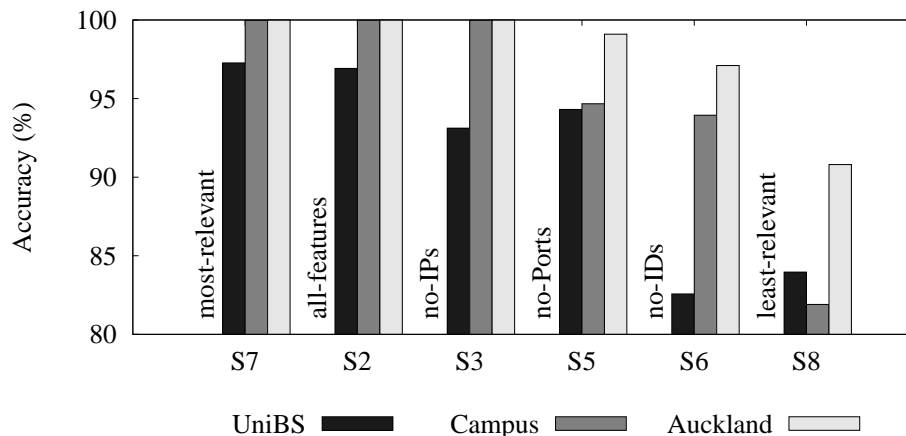
Figure 13. Flow classification accuracy for different traces and features sets (homogeneous training, k = 100 sampling).
