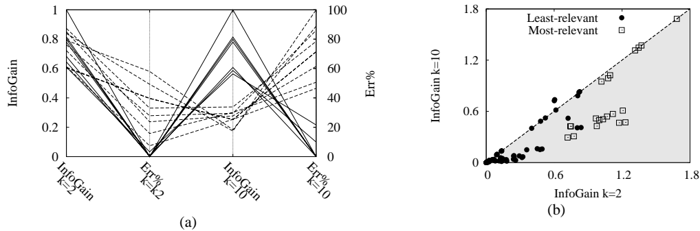
Figure 10. (a) Parallel coordinates plot for most-relevant features and (b) scatter plot of information gain for all features with k = 2, 10 .
