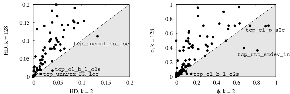
Figure 5. Scatter plot of Hellinger distance and \phi coefficient over the whole features set for systematic sampling with k \in \{2, 128\} .
