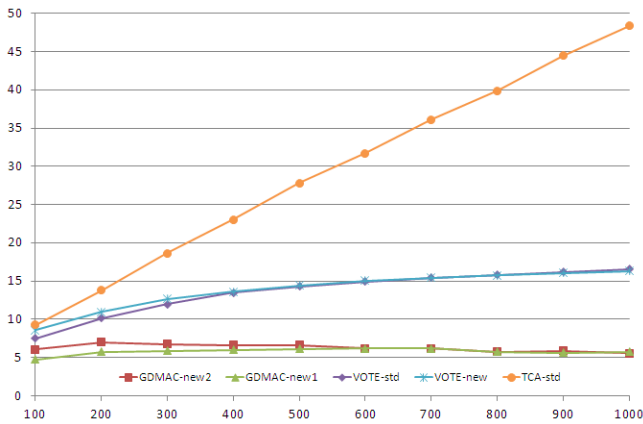
Fig. 1. Average cluster size vs. N in static networks.
