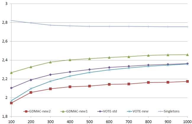
Fig. 3. J vs. N in static networks.
