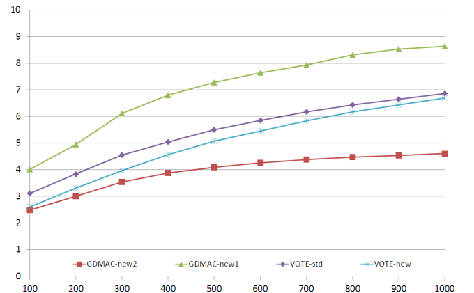
Fig. 2. Group cluster diversity vs. N in static networks.
