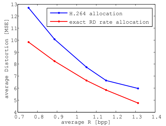
(b) Sequence coastguard .
