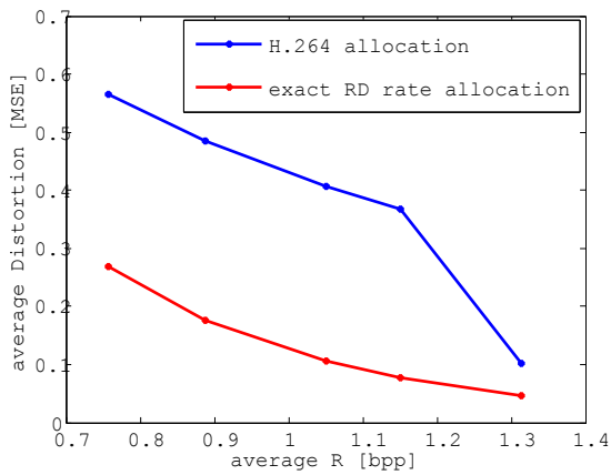
(a) Sequence akiyo .
