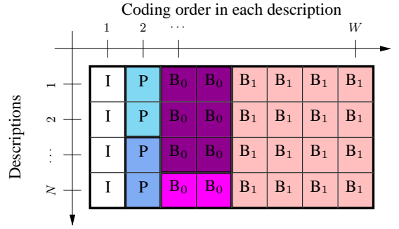
Fig. 3. Example of MD-GOP clustering. Frames in the same cluster share similar RD properties.
