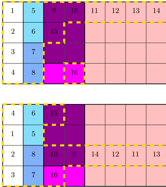
Fig. 4. Two possible schedules (first 16 packets). The numbers indicate the order in which the frame is included in the coding window. The dashed border identifies which frames have been selected for inclusion in the coding window at the 16-th packet.
