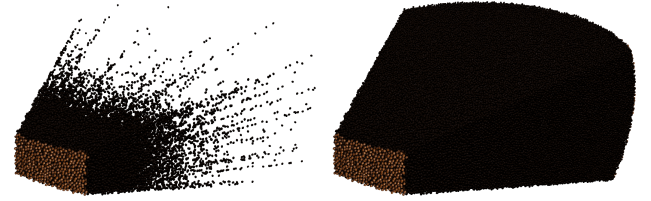
Figure 14: View frustum with (left) and without (right) our grain occlusion culling. Some of the remaining points may actually be hidden, but it is ensured that no visible point is removed.
