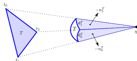
Fig. 1. Triangle T projected on the spherical triangle \bar{T} .
