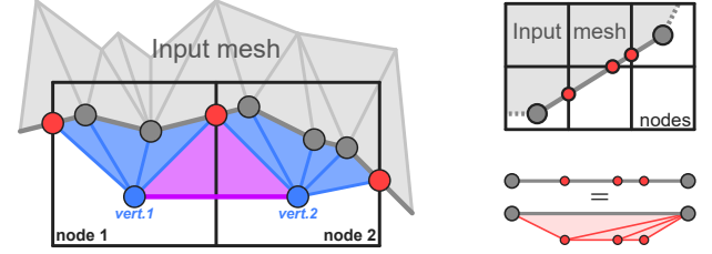
Figure 4: With boundary vertices in gray, node vertices in blue, and intersection vertices in red, we add blue triangles inside nodes, and purple triangles between nodes sharing a vertex, and “subdivide” edges by adding 0-area triangle fans (right).
