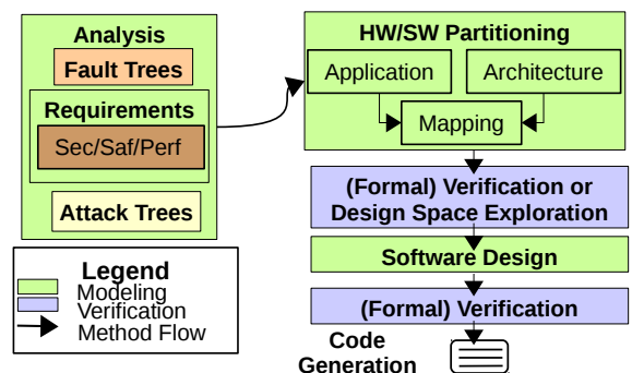
Figure 1: SysML-Sec modeling profile used in TTool.
