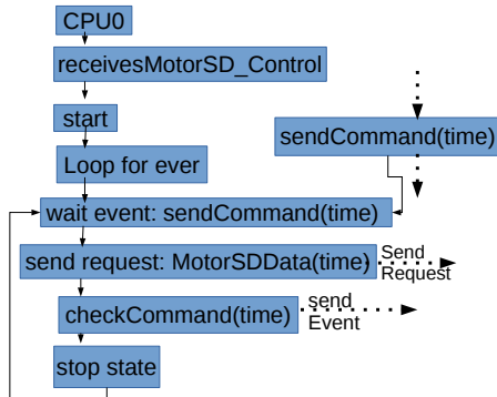
Figure 6: Excerpt of the Latency Graph
