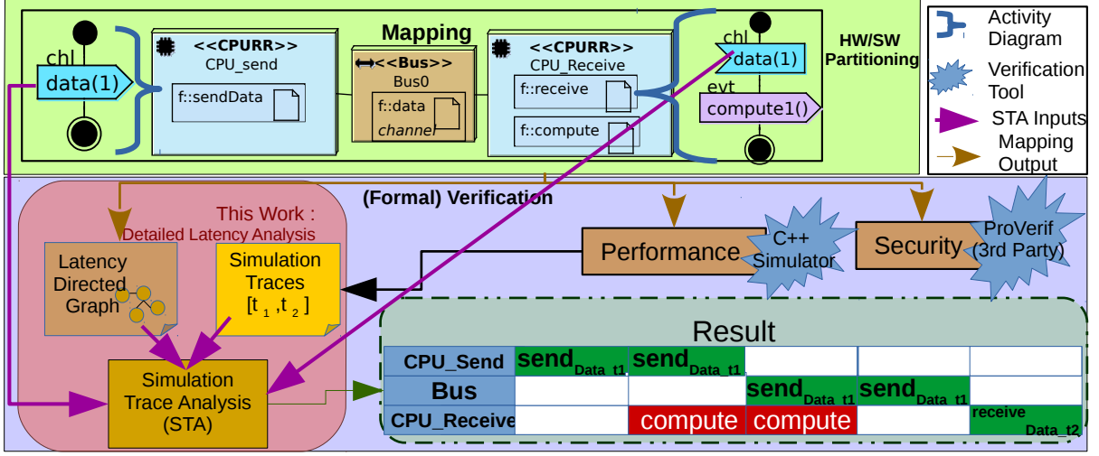
Figure 2: Detailed Latency Analysis Method added to SysML -sec.
