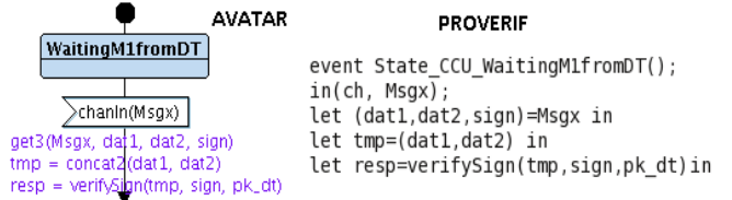
Figure 4. Five elements in an AVATAR-ProVerif translation
