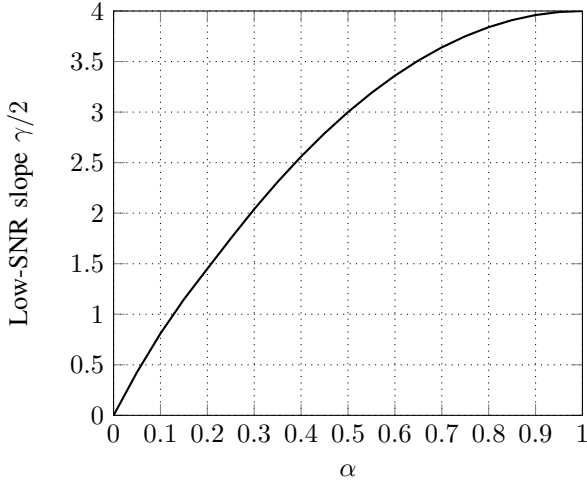
Fig. 3. The low-SNR asymptotic slope \gamma/2 , see (50), is depicted as a function of \alpha \in (0, 1) for the two-LED MISO channel with gains h_1 = 3 and h_2 = 1 (the same channel as considered in Figure 2).
