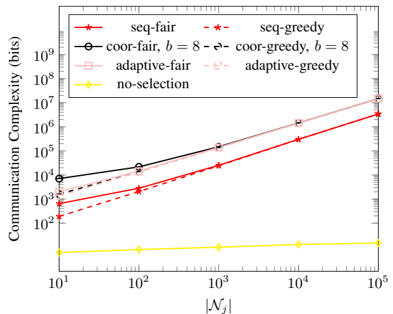
Fig. 7: Lower bound on the communication complexity of each strategy in function of |\mathcal{N}_j| . Here, k = 100 and G = 10 .
