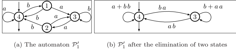
FIGURE 6. The state elimination method on the automaton \mathcal{P}'_1
