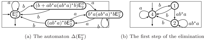
FIGURE 9. Running the algorithm with a smart ordering
