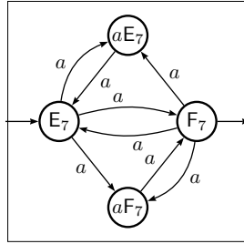
(a) The automaton \Delta(E_7)
