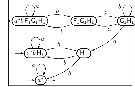
FIGURE 3. The derived term automaton of E_1 = a^* + a^*b(ba^*b)^*ba^* + a^*b(ba^*b)^*a(b + a(ba^*b)^*a)^*a(ba^*b)^*ba^*
