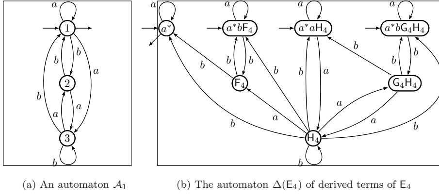
FIGURE 4. The core of the algorithm
