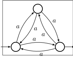
(b) The automaton \mathcal{A}_7
