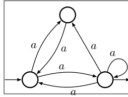
(c) Another characteristic \mathbb{N} -co-quotient
