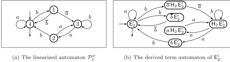
FIGURE 7. The complete algorithm on automaton \mathcal{P}'_1
