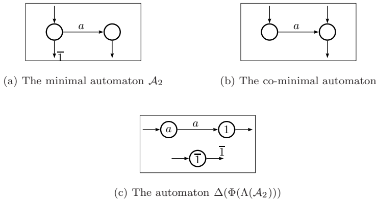
FIGURE 8. Three automata that recognize 1 + a
