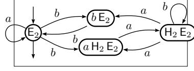
FIGURE 2. The derived term automaton of E_2 = (a + bb + ba(b + aa)^*ab)^*
