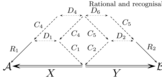
Fig. 14. Structural decomposition of the equivalence of two \mathbb{K} -automata
