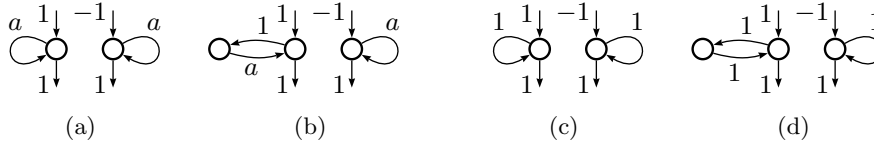
Fig. 6. Advocating for a path-based definition of the behaviour of automata
