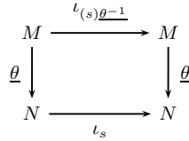
Fig. 12. Lifting of \mathbb{K} -intersection with s
