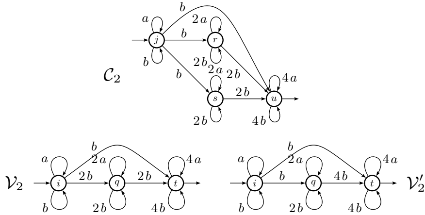
Fig. 9. \mathcal{C}_2 is an \mathbb{N} -covering of \mathcal{V}_2 and a co- \mathbb{N} -covering of \mathcal{V}'_2
