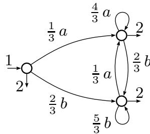
Fig. 7. The \mathbb{Q} -automaton \mathcal{S}_{E_1}
