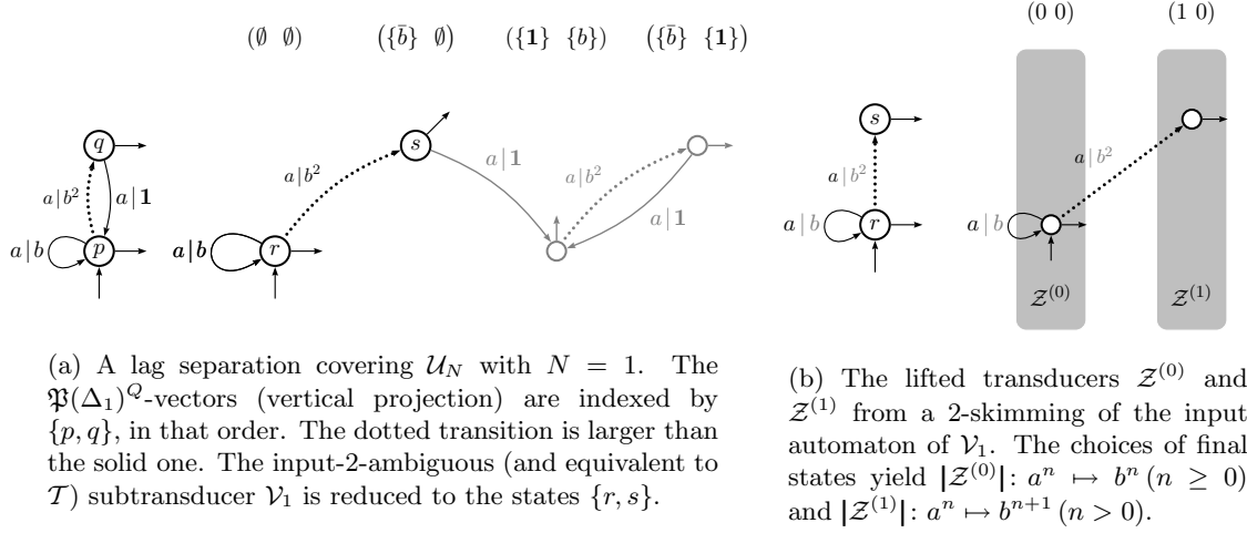
Figure 6: A decomposition of the 2-valued transducer \mathcal{T} of Figure 2.
