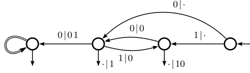
Fig. 2. The successor function for the Fibonacci numeration system
