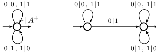
Fig. 3. A synchronized transducer for the radix order relation on A = \{0, 1\}
