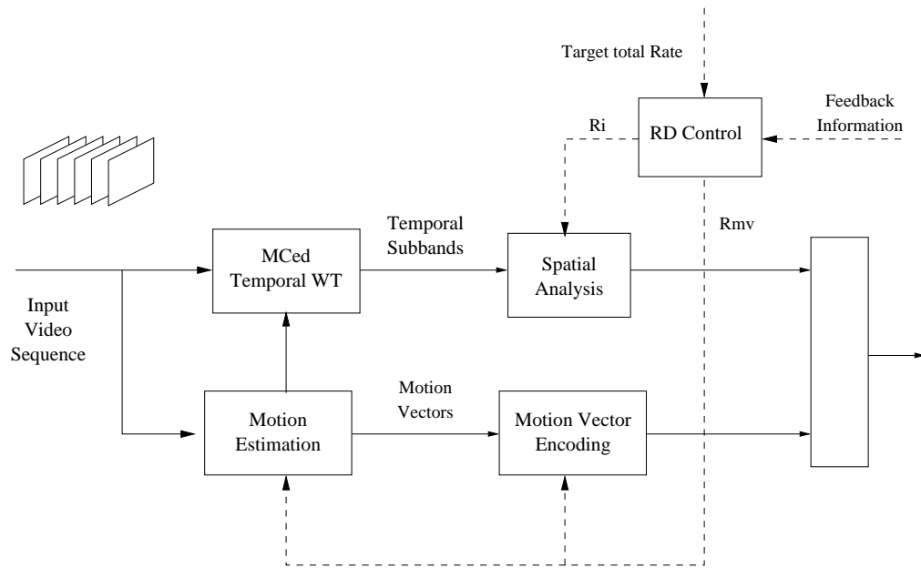
Figure 7.1: Global coding scheme
