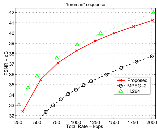
Figure 6.8: Compression performance of the proposed encoder on the “foreman” sequence
