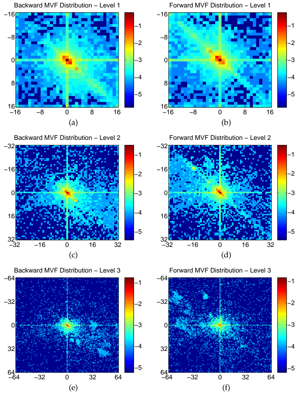
Figure 5.5: MVF distribution: "foreman", full pixel
