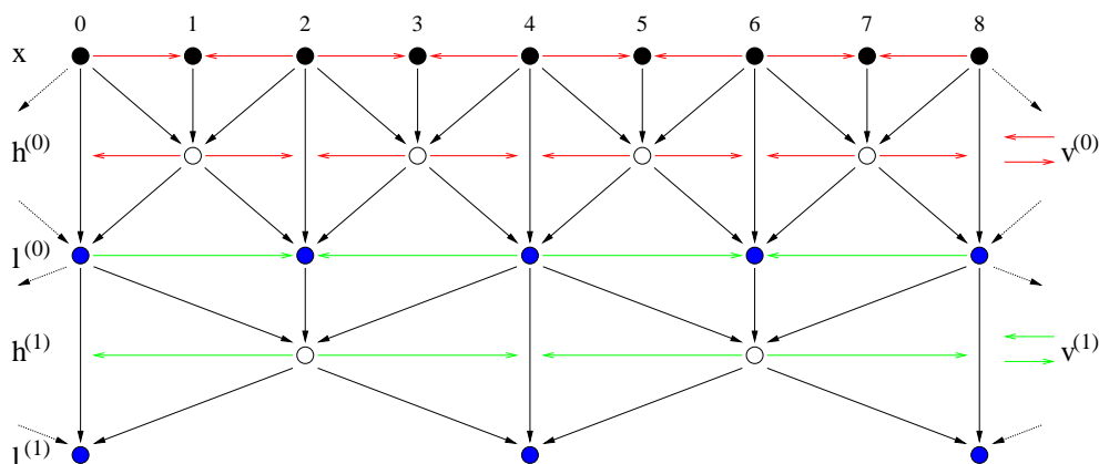
Figure 4.7: Scheme of a two-level temporal decomposition with the (2, 2) LS. In this case V_1 = \{\mathbf{v}^{(0)}, \mathbf{v}^{(1)}\} .
