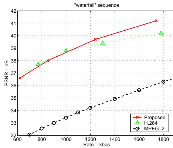
Figure 6.9: Compression performance of the proposed encoder on the “waterfall” sequence
