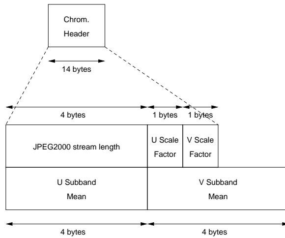
Figure C.7: Chrominance image header structure
