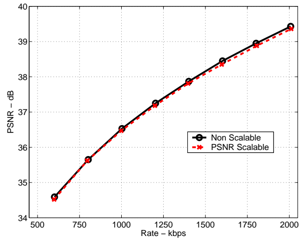
Figure 6.5: Cost of SNR scalability
