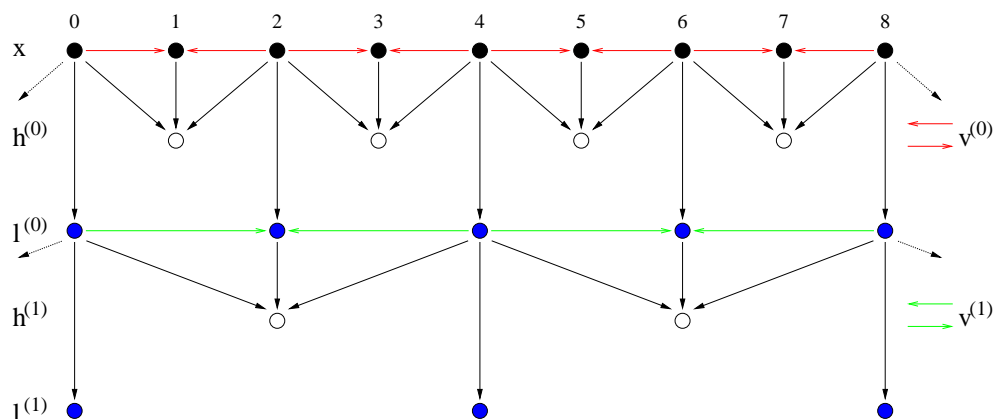
Figure 4.8: Scheme of a two-level temporal decomposition with the (2, 0) LS. In this case V_1 = \{\mathbf{v}^{(1)}\} , as h_k^{(1)} is computed directly from x_k independently from h_k^{(0)}
