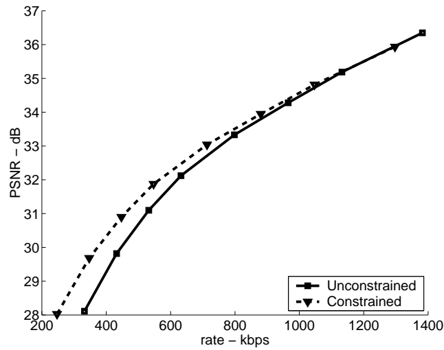
Figure 4.6: Impact of ME methods on codec performance
