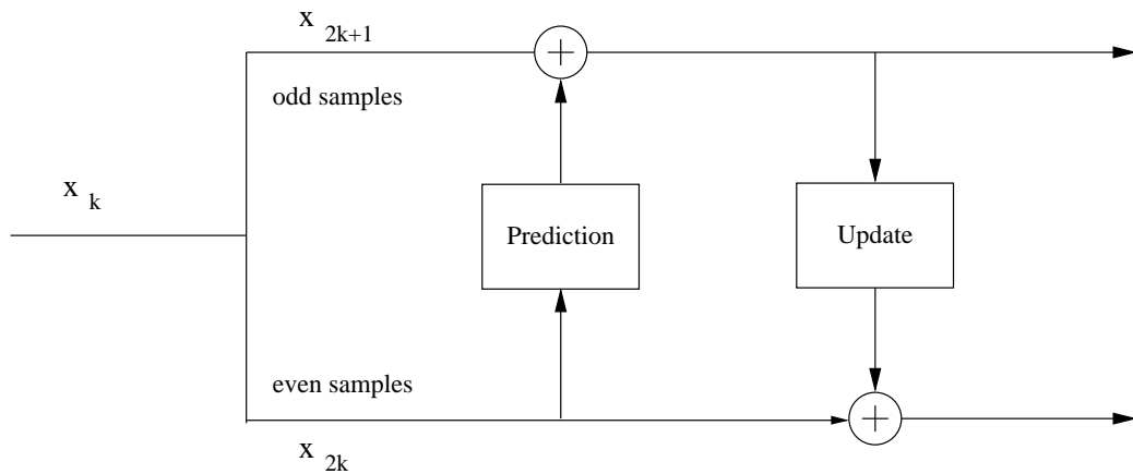
Figure 3.2: A single lifting stage of a lifting scheme
