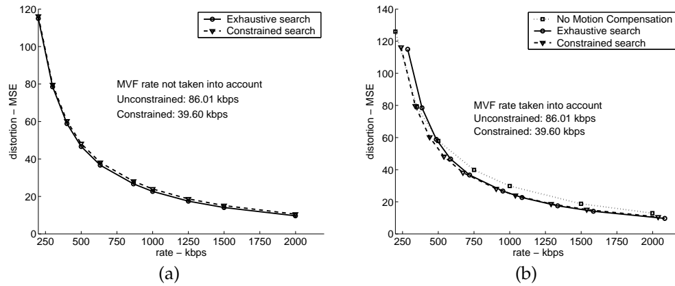
Figure 4.3: Comparison between ME methods (a) and their impact on codec performance (b)
