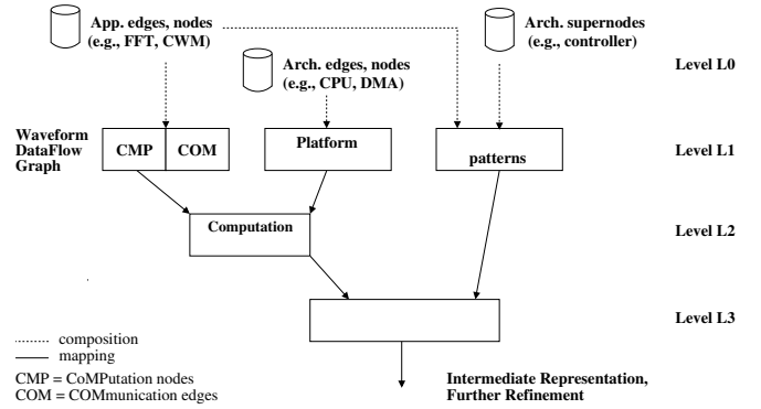
Fig. 4. The proposed modeling approach
