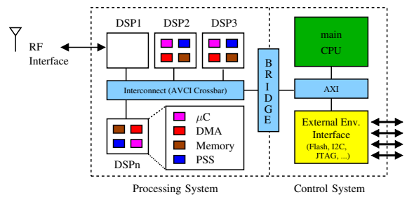
Fig. 1. The architecture of an Embb instance
