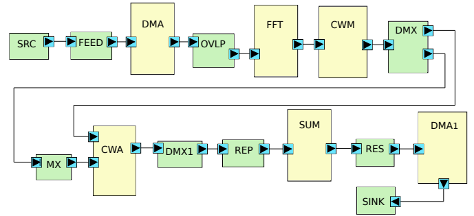
Fig. 7. WPD waveform DataFlow Graph of level L1 adapted to Embb
