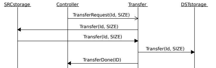
Fig. 3. An abstract communication pattern
