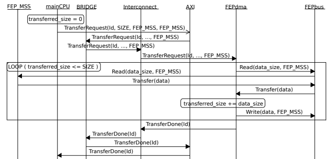
Fig. 5. The Communication Pattern of Fig. 3, after mapping level L3
