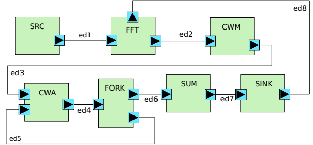
Fig. 6. WPD waveform DataFlow Graph of level L1
